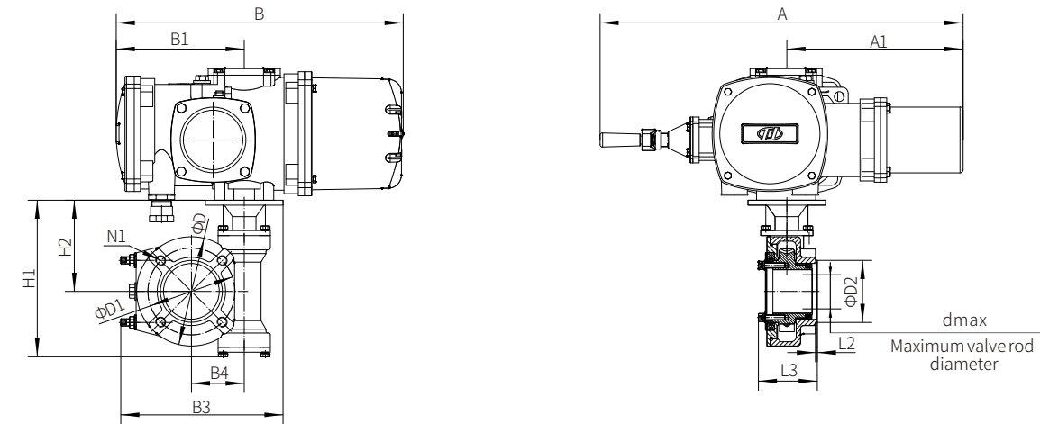
c) Connecting dimension of directly-connected gearbox
