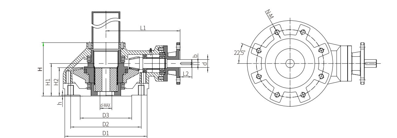
c) Boundary and mounting dimensions
